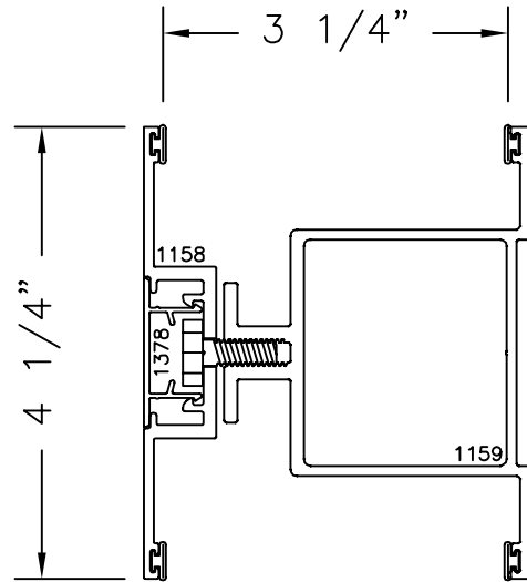
3 1/4" PARTITION COMPRESSION MULL
