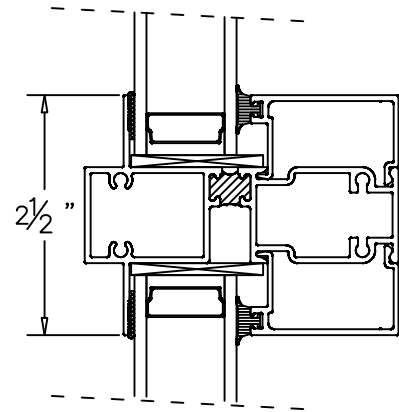
SERIES 700 & 4100 FIXED
