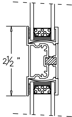
SERIES 500 & 700 OPERATING
